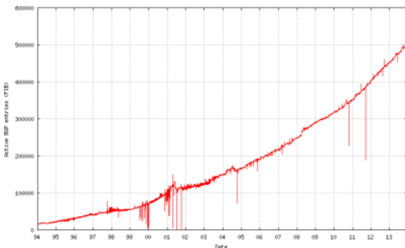
Figure 1. Active BGP entries
