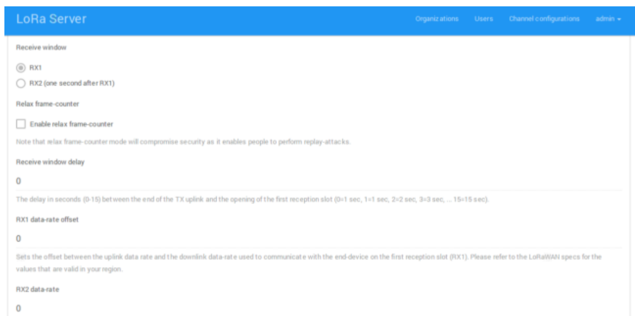
Figure 3. Receive window selection on lorasever backend
