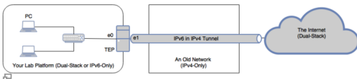
Figure 2. 6in4 Tunnel for extending IPv6 connectivity
